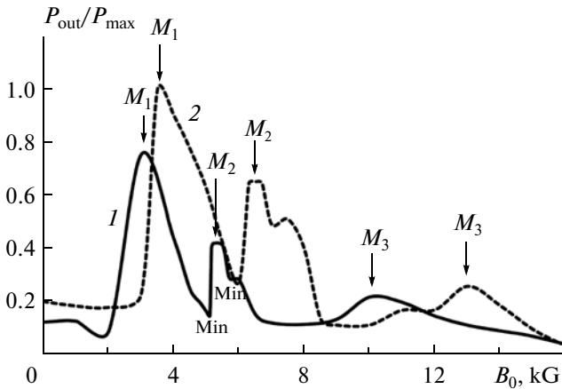
Fig. 1. Dependences of the normalized output power of radiation from REBs with VCs on the induction of external magnetic field B_0 at the following values of initial beam energy W_e : 600 keV (curve 1) and 850 keV (curve 2). Beam current, I = 20 kA; symbols M_1 , M_2 , and M_3 denote the local maxima of the dependences.
