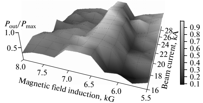
Fig. 2. Dependences of the normalized output power of radiation from REBs with VCs on the induction of an external magnetic field and beam current. W_e = 850 keV.
